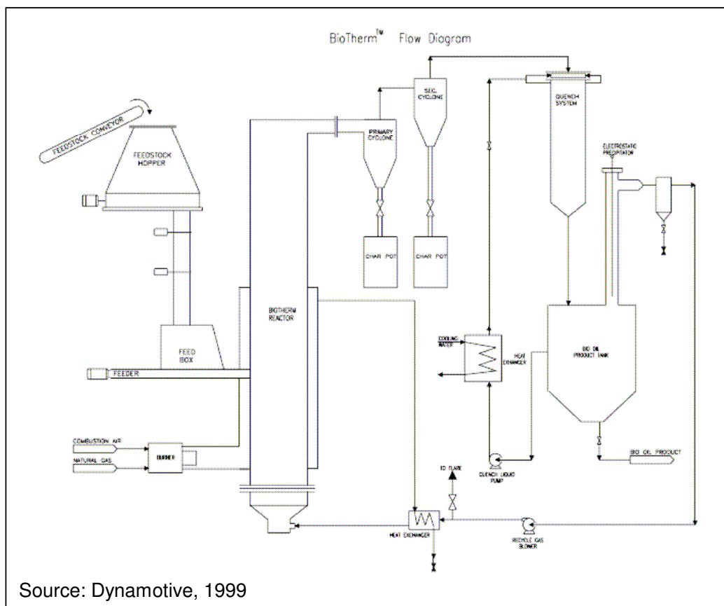
Figure 12. Biotherm Process Flow Diagram
