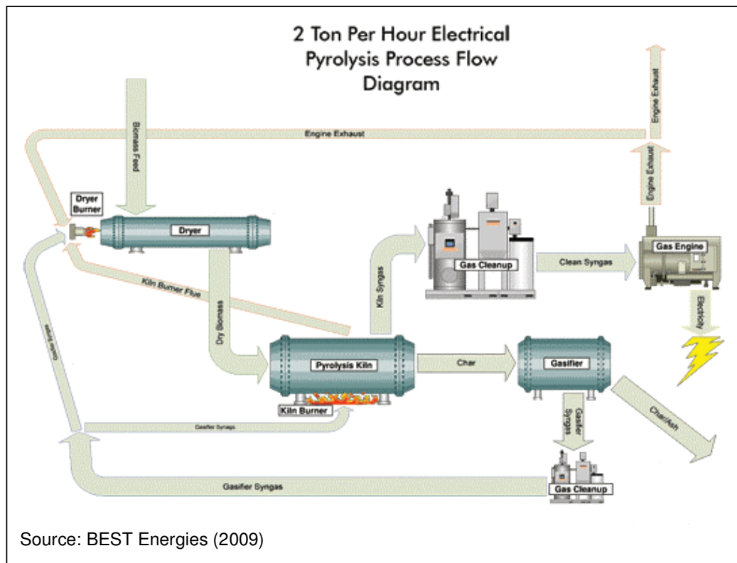
Figure 10. BEST Energies Slow Pyrolysis Plant: Outline Process Flow
